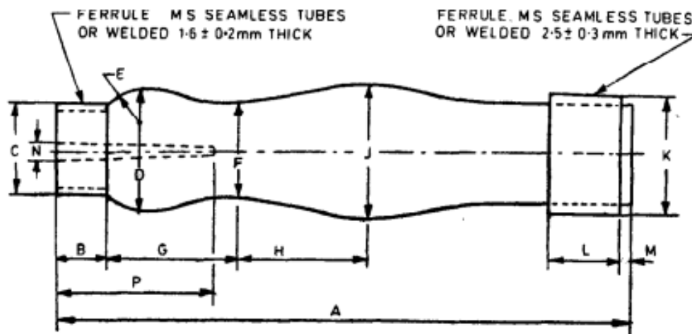
Fig. 1 Typical Sketch of Wooden Handle for Chisels and Gouges
